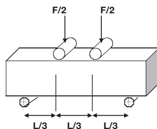
Apply load = 50% residual load at 5mm
