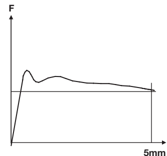
Apply load = 50% residual load at 5mm
